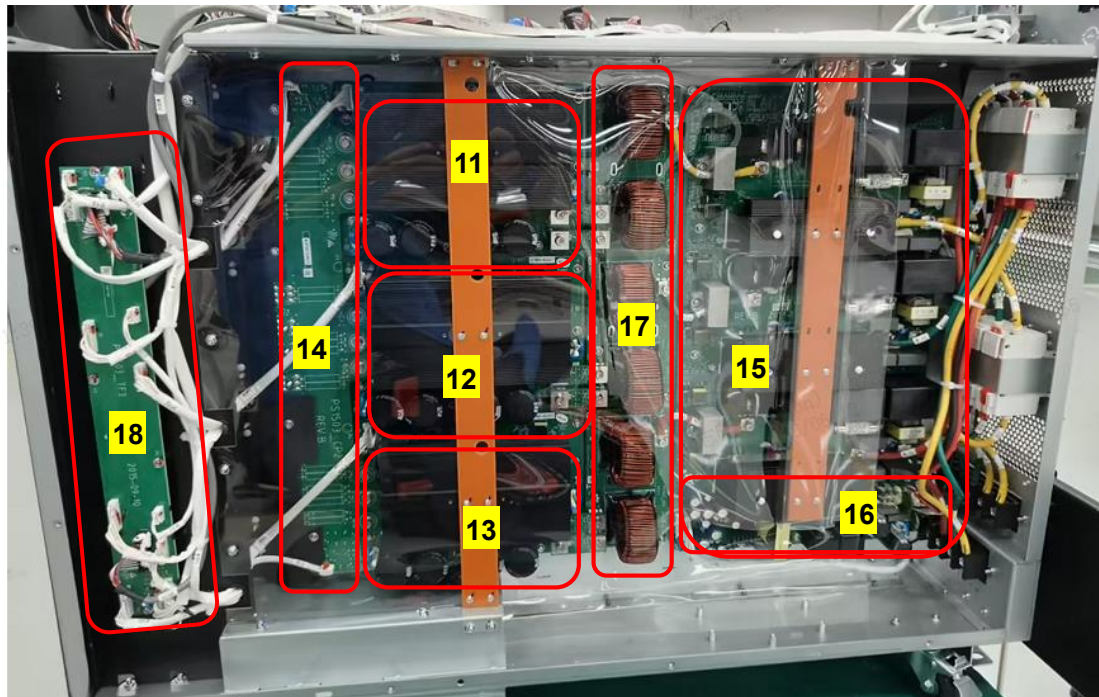
Fig.1-3 Left side structure
