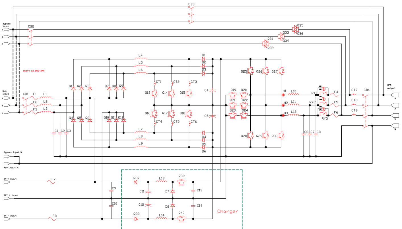
Fig.2-2 DT33030XL topology
