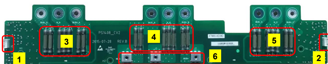
Fig.3-16 Inverter bus board introduction
