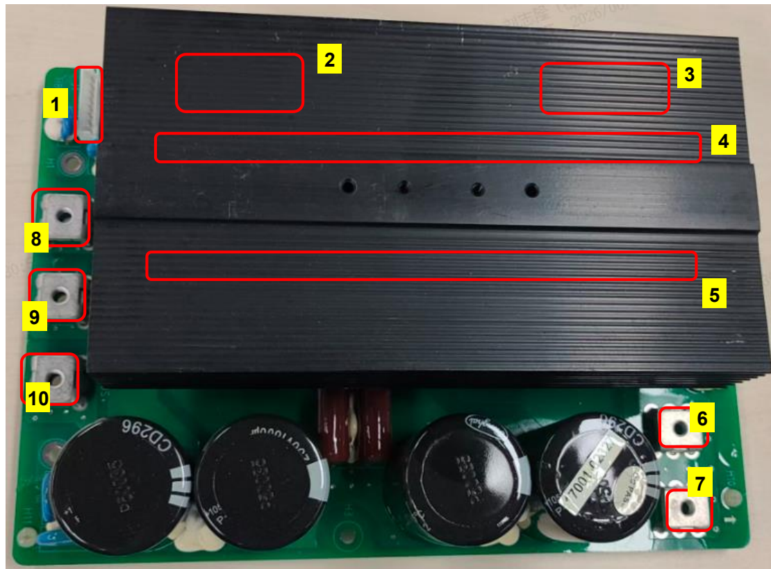
Fig.3-10 Inverter board introduction
