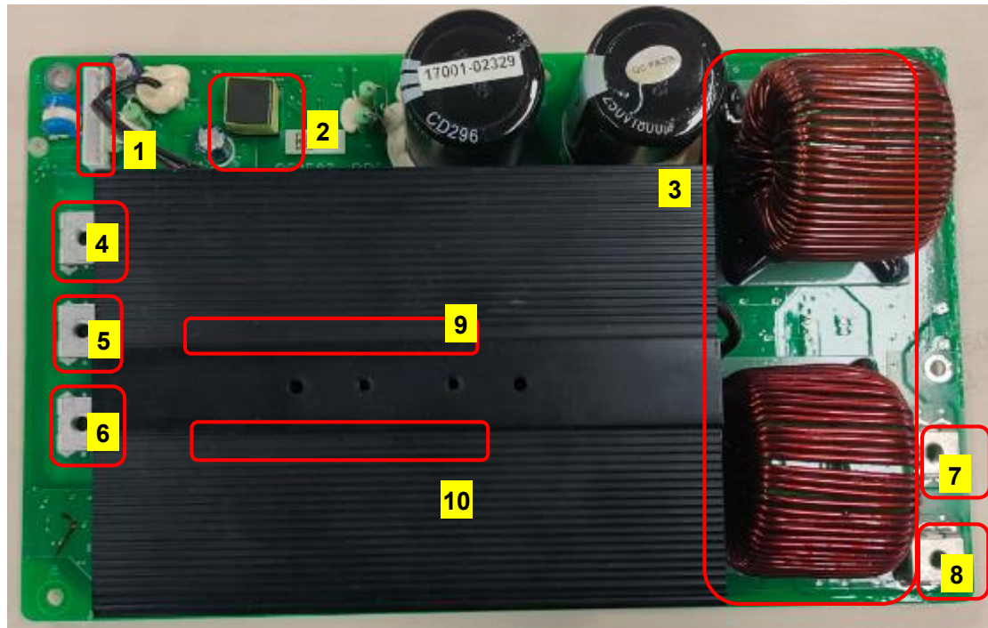
Fig.3-8 PFC board introduction
