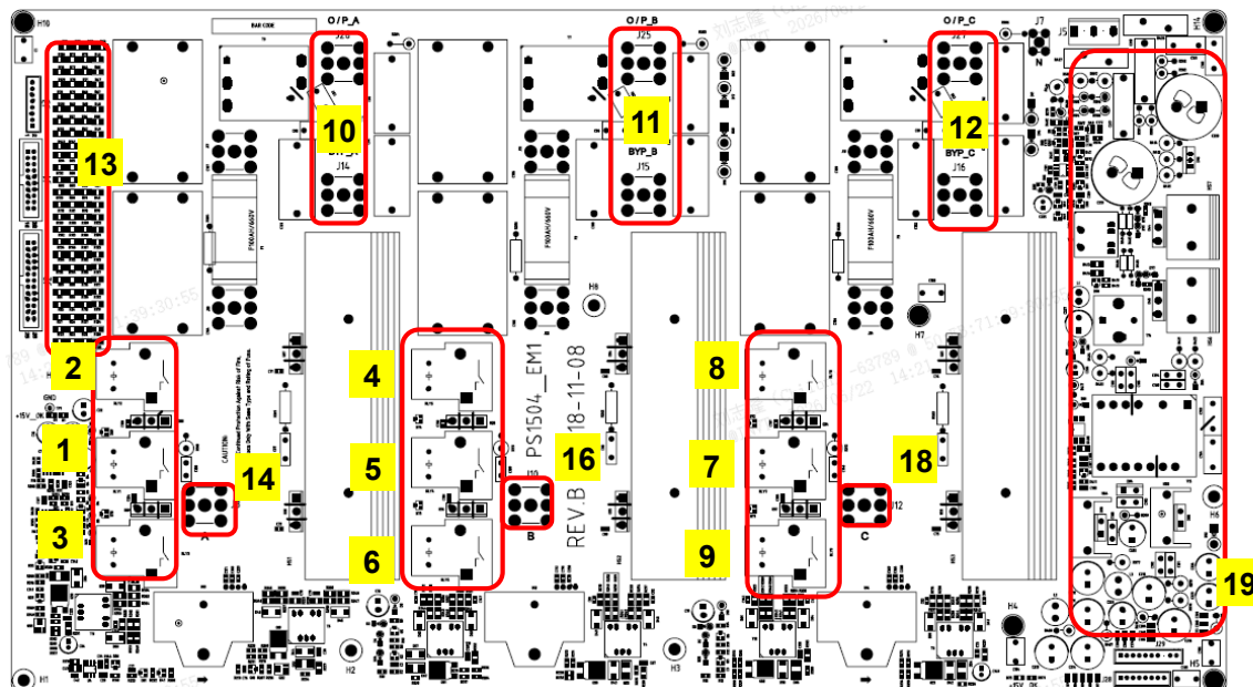
Fig.3-13 Output board assembly diagram
