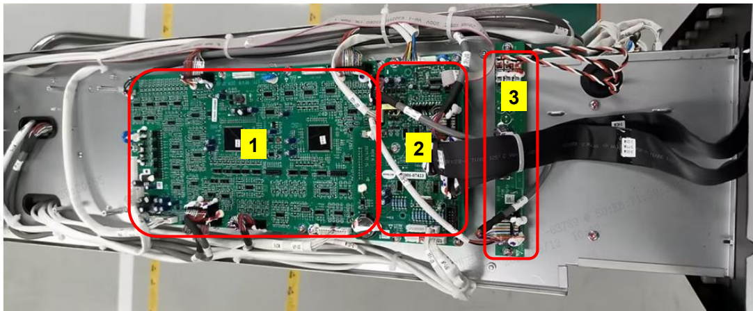
Fig.1-1 Top side structure
