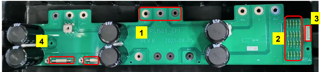
Fig.3-18 Rectifier bus board introduction
