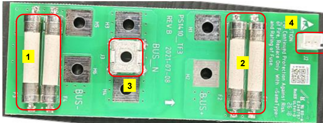
Fig.3-20 Inverter bus board introduction
