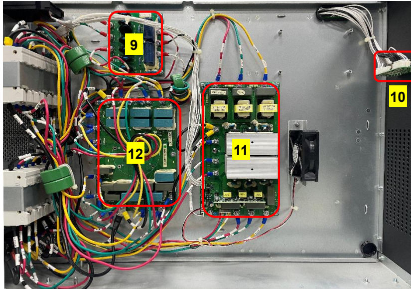
Fig.1-3 Left side structure
