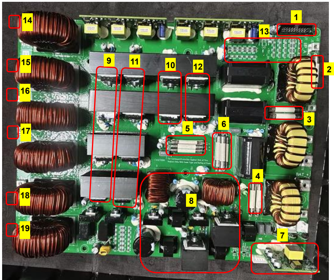
Fig.3-3 Input SCR board introduction
