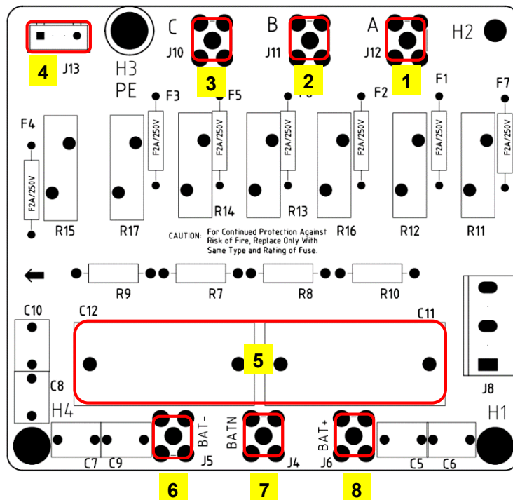
Fig.3-27 Battery EMI and lighting protection board assembly diagram
