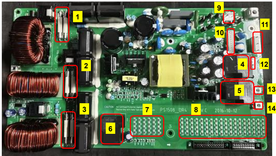
Fig.3-14 Output board introduction
