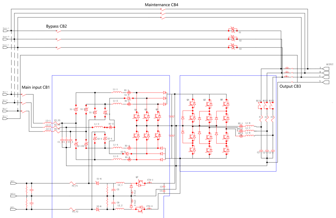
Fig.2-2 DT33010XL topology
