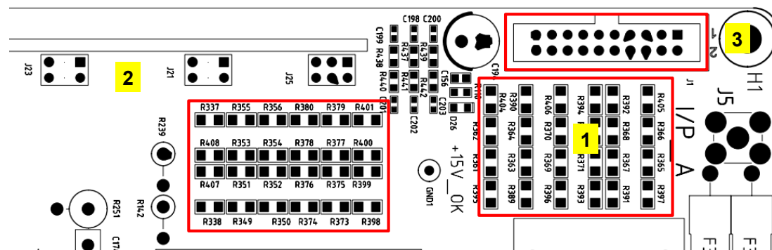
Fig.3-5 Sampling detect introduction
