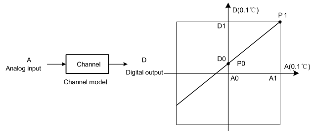
Figure 3-1 IVC1L-2TC channel characteristic setting
