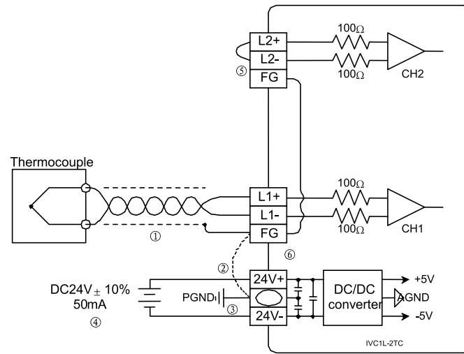
Figure 1-4 Wiring of IVC1L-2TC user port
