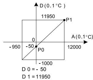
Figure 3-3 Changing characteristic
