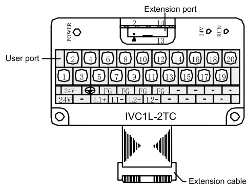
Figure 1-2 IVC1L-2TC ports
