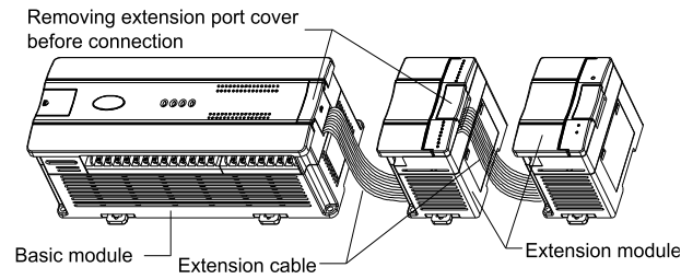
Figure 1-3 Connecting into system
