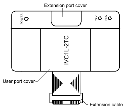
Figure 1-1 IVC1L-2TC appearance
