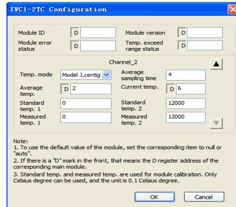
Figure 4-2 CH2 setting interface
