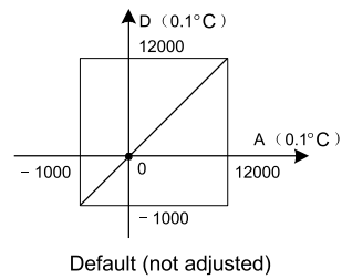
Figure 3-2 Characteristic of 0 mode without changing D0 and D1
