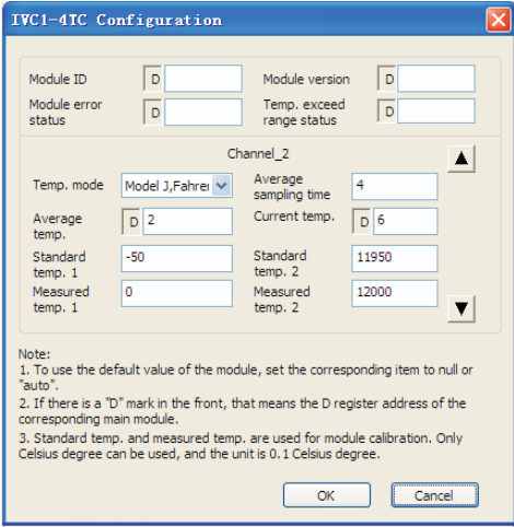
Figure 4-6 Changing CH2 characteristic
