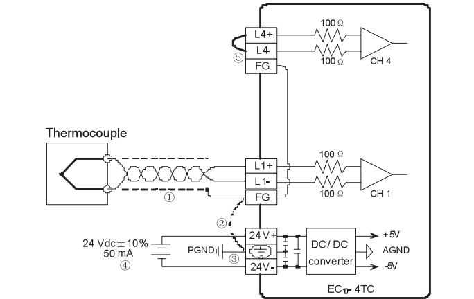
Figure 1-4 Wiring of IVC1-4TC user port
