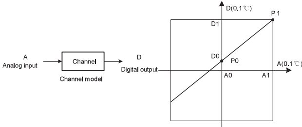
Figure 3-1 IVC1-4TC channel characteristic setting
