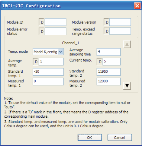
Figure 4-5 Changing CH1 characteristic
