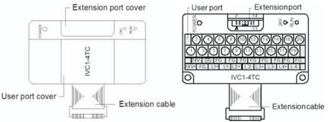
Figure 1-1 IVC1-4TC appearance
